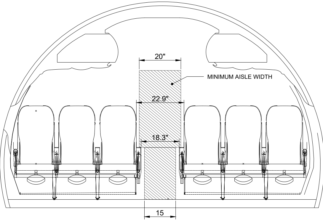
FIGURE 3-C1. CONSTANT SECTION FRONT VIEW - MINIMUM AISLE WIDTH REQUIREMENTS, FRONT ROW SEATS
